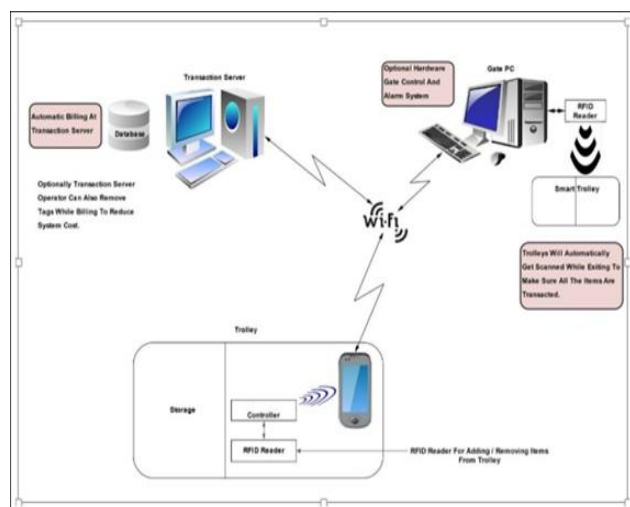
Fig 2. System architecture
